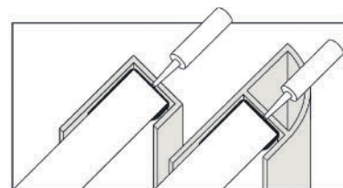
Square and Quadrant End Trims
