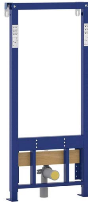
Wall Hung Bidet Frame 500 x 1140-1180 x 135-200 £219.00
