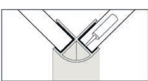
External Corner Used on all external 90° corners.
