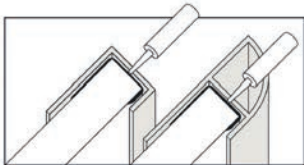
End Trims and Quadrant Trims Finishing end trims for square cut edge panels.
