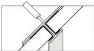
Jointing Trim - For Square Cut Only Used to mount panels side by side.
