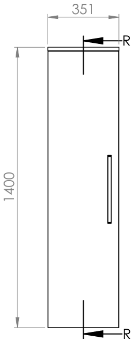
FRONT VIEW
