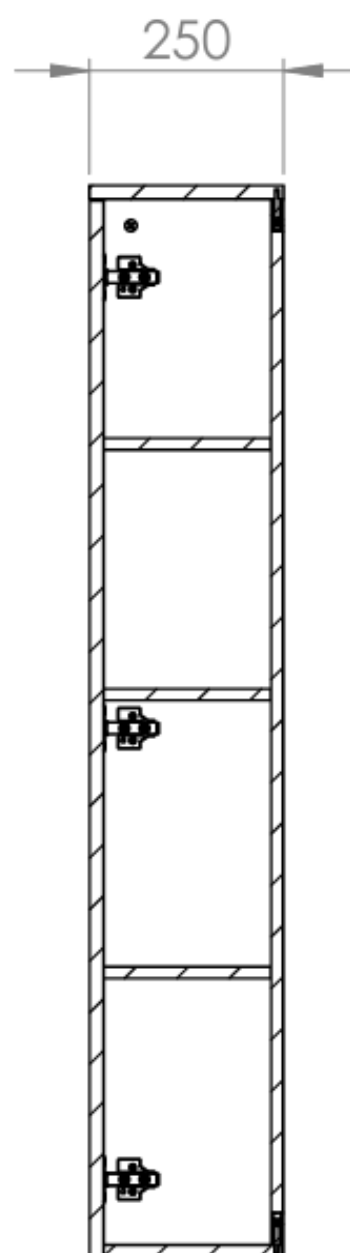
SIDE VIEW
