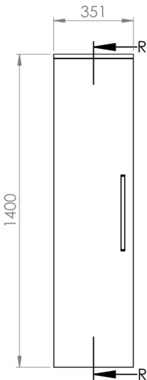
FRONT VIEW
