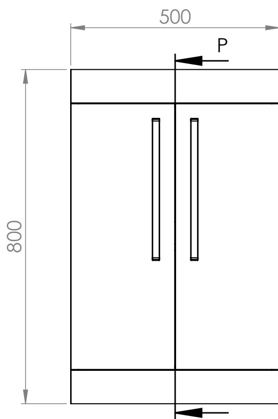
FRONT VIEW
