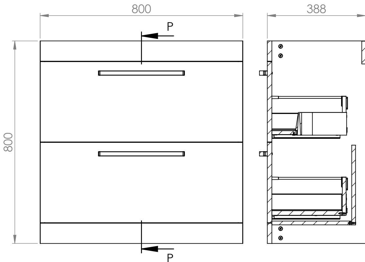
FRONT VIEW
