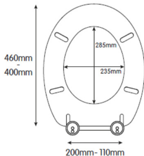
Max/Min Adjustment
