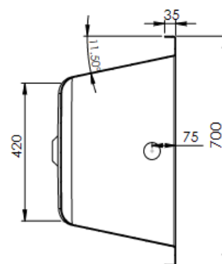
SECTION F-F SCALE 1 : 10
