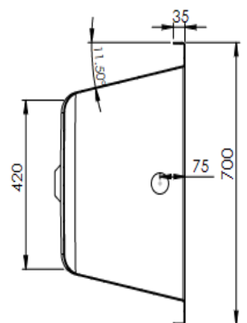
SECTION F-F SCALE 1 : 10
