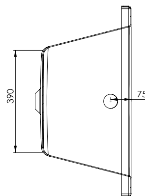
SECTION L-L SCALE 1 : 7
