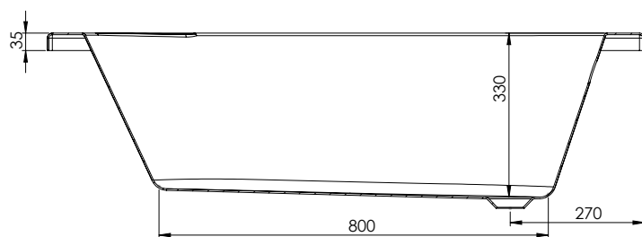
SECTION M-M SCALE 1 : 7
