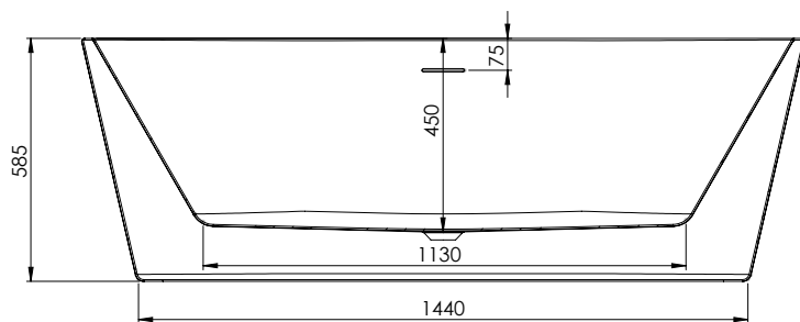
SECTION K-K SCALE 1 : 10
