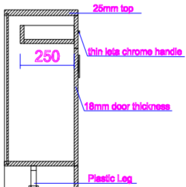
SIDE AA SECTION VIEW
