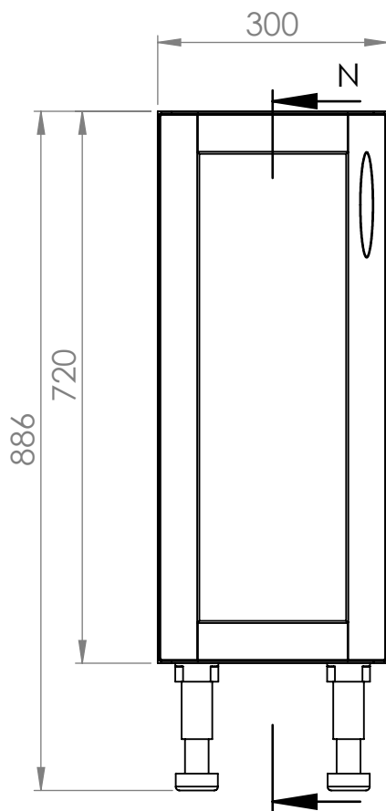
FRONT VIEW
