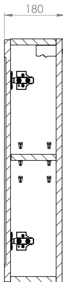
SIDE VIEW
