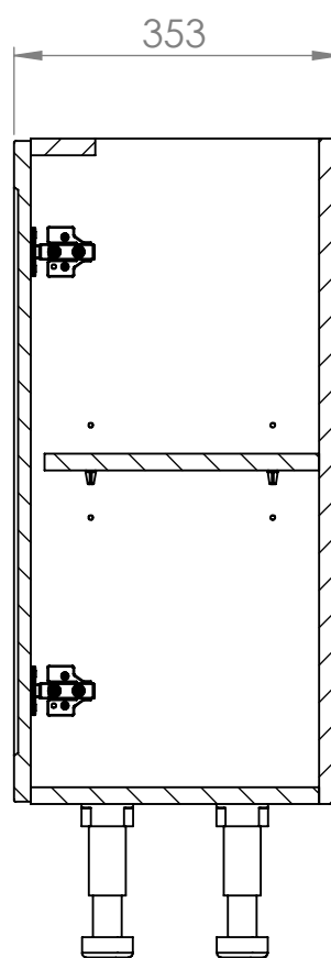
SIDE VIEW
