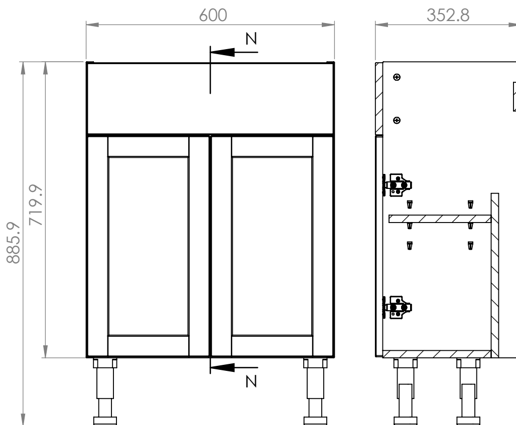
FRONT VIEW
