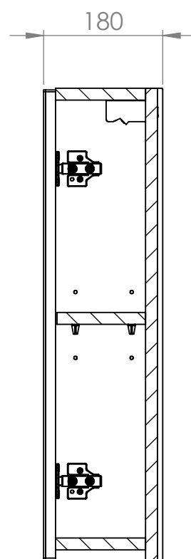
SIDE VIEW
