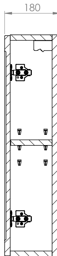
SIDE VIEW
